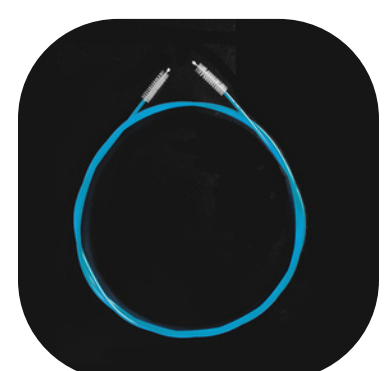
CODE: CB-40-8 TOTAL LENGTH: 2300 mm BRUSH LENGTH: 20 mm BRUSH DIMETER: 6 mm
