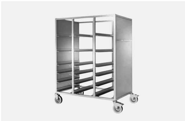
Code T1-10-7 Material : Stainless Steel Feet : 4 wheels - 2 braked Package : 1 Piece Dimensions: 700 x 360 x 1350 mm (W x L x H)
